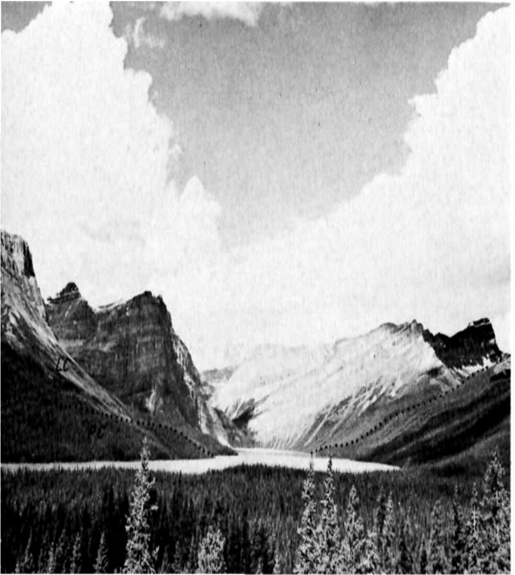
Figure 32. Hector Lake, west of the Banff-Jasper highway, is fed by glaciers along the Continental Divide. The cliffs are Middle Cambrian limestones dipping west away from the centre of Bow anticline.
