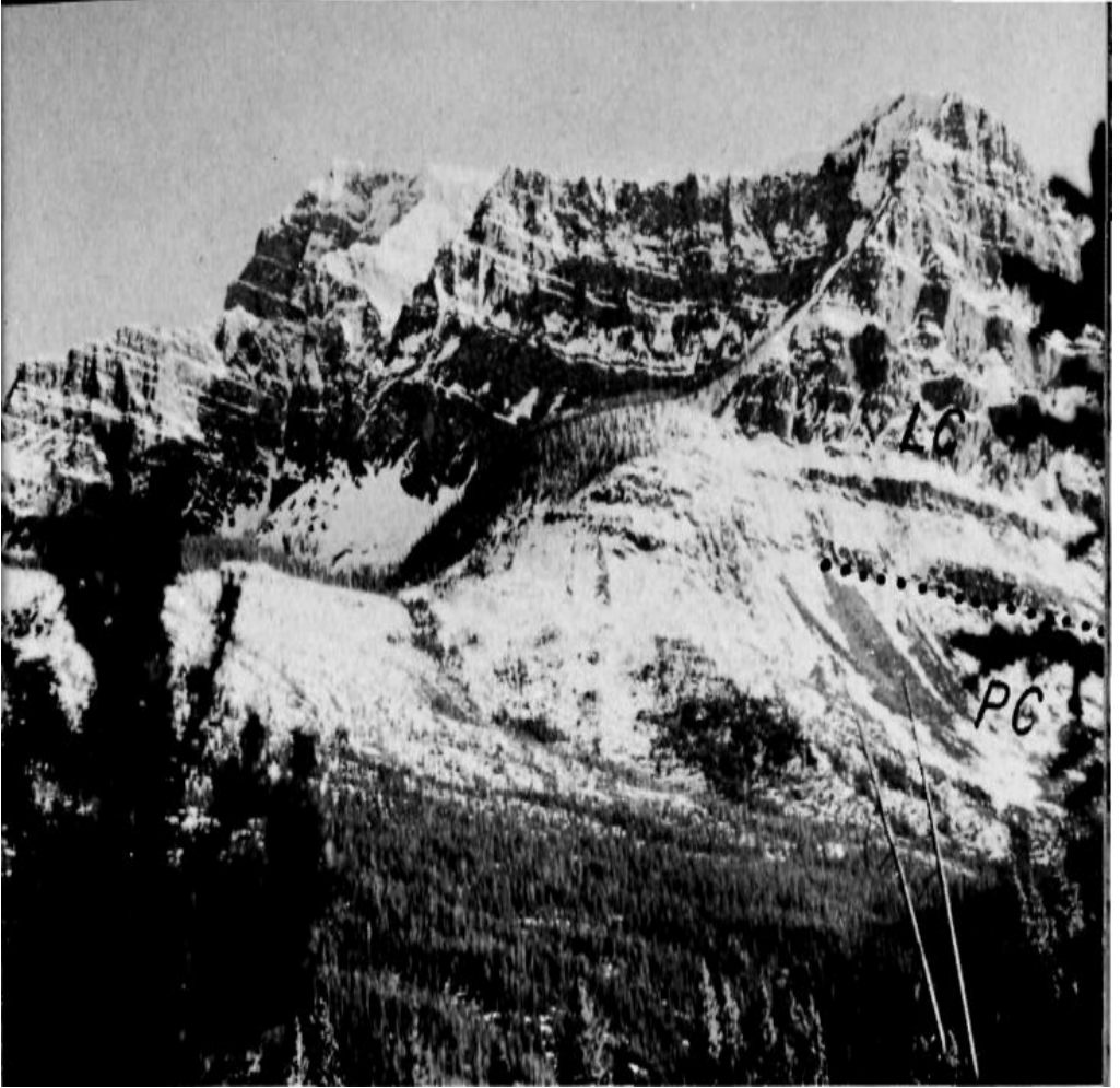
Figure 2. Ridges of Storm Mountain from Vermilion Pass, Banff-Windermere highway. Hard beds of rock stand up as cliffs and soft shale layers weather back, emphasized here by the light snow covering. Aglacier caps the ridge. PC, Precambrian shales; LC, Lower Cambrian quartzites and shales.
