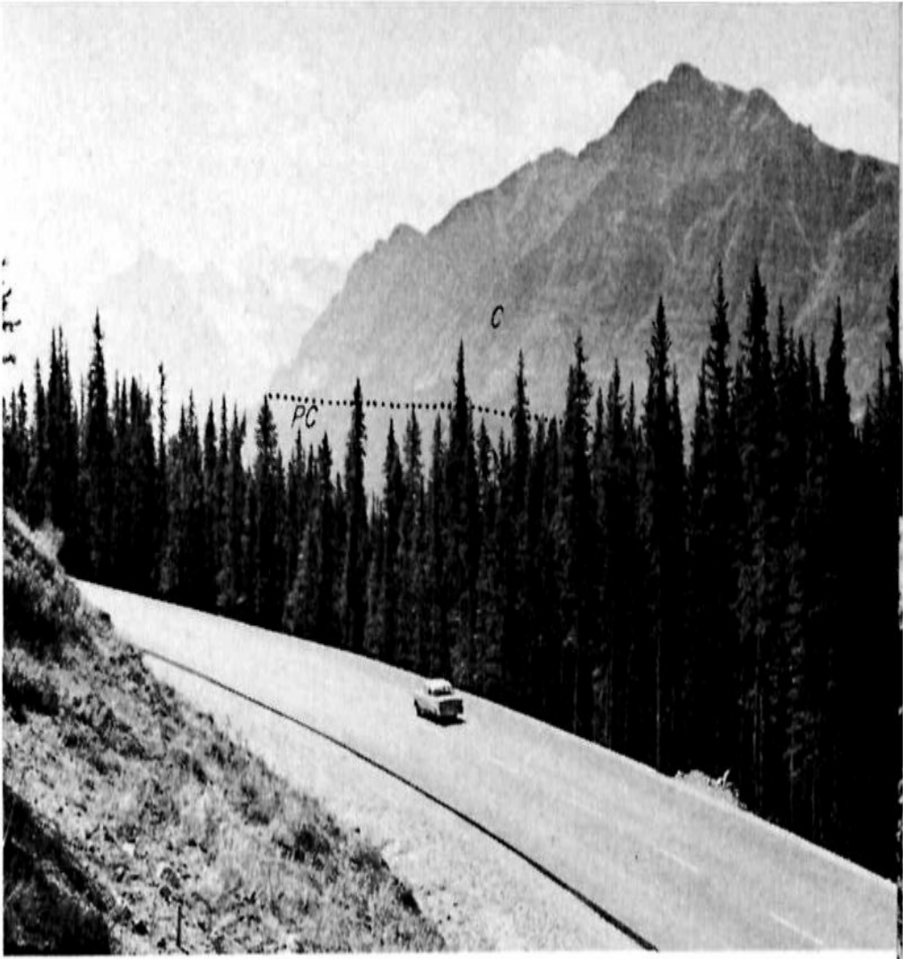
Figure 29. The Waputik Range and mountains in the Lake Louise area. The rugged cliffs are mostly Cambrian limestones (C) and the lower slopes Precambrian (PC) shales.
