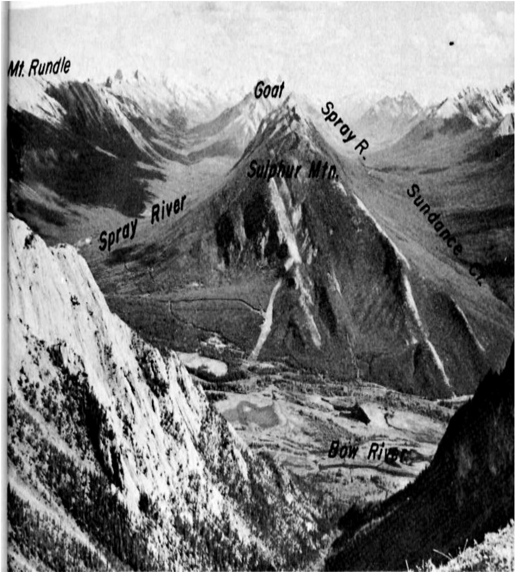
Figure 25. Sulphur Mountain, Spray and Sundance valleys from
