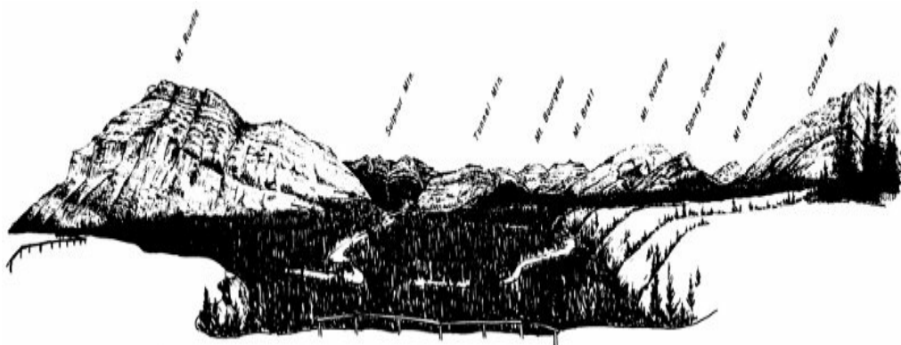
Figure 26. Sketch of view from Hoodoos Viewpoint. You look directly west up Bow River valley. The road follows the river across the mountain range. These ranges are thrust blocks of which the scarps face east and the rock layers dip westward. The terraces on which you stand and on either side of the valley are glacial drift.
