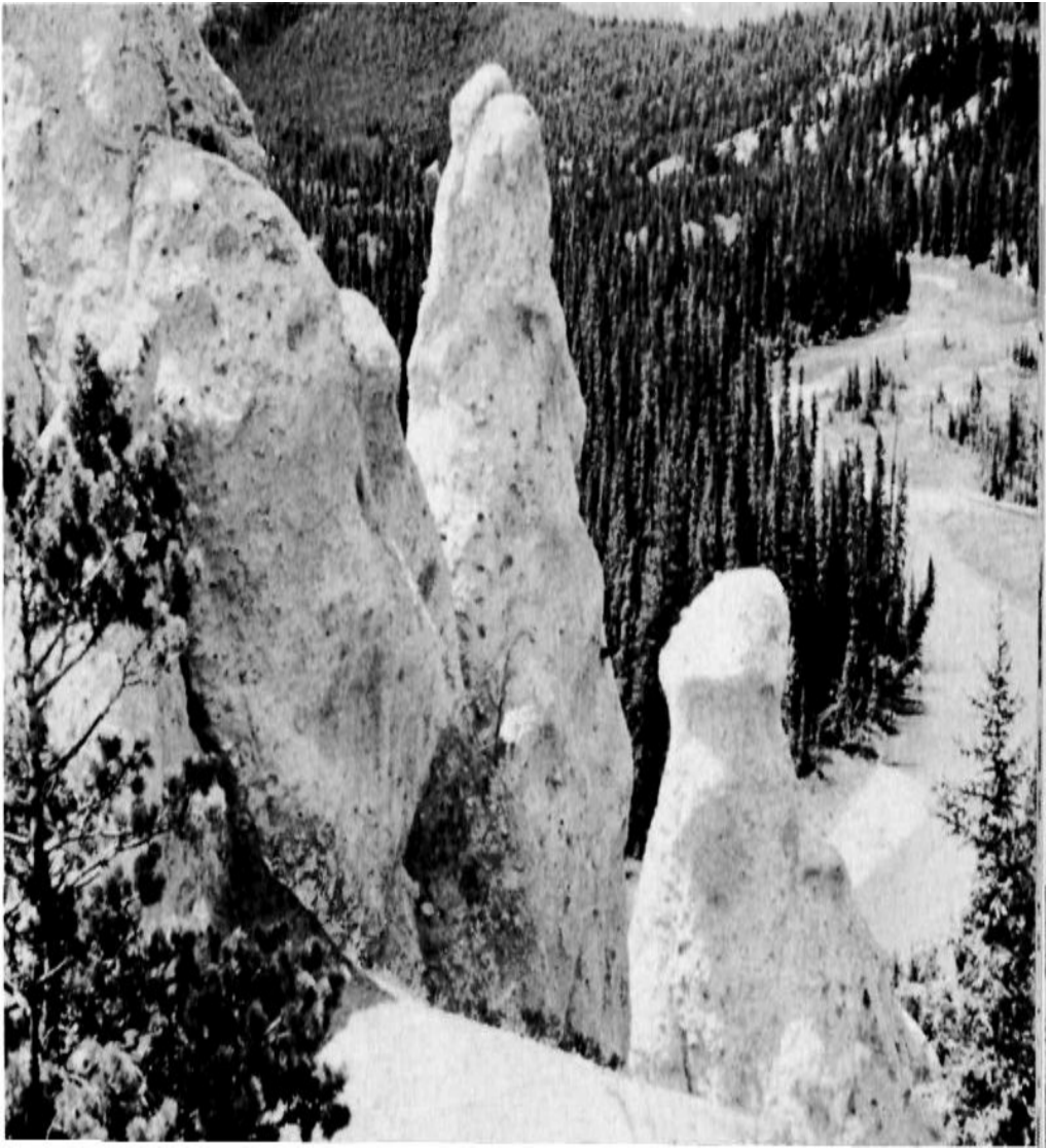
Figure 16. The Hoodoos at the Hoodoos Viewpoint, Banff. The Hoodoos are formed of cemented glacial till composed of mud, sand and scattered stones left behind by the glacier that once flowed down the Bow River valley.
