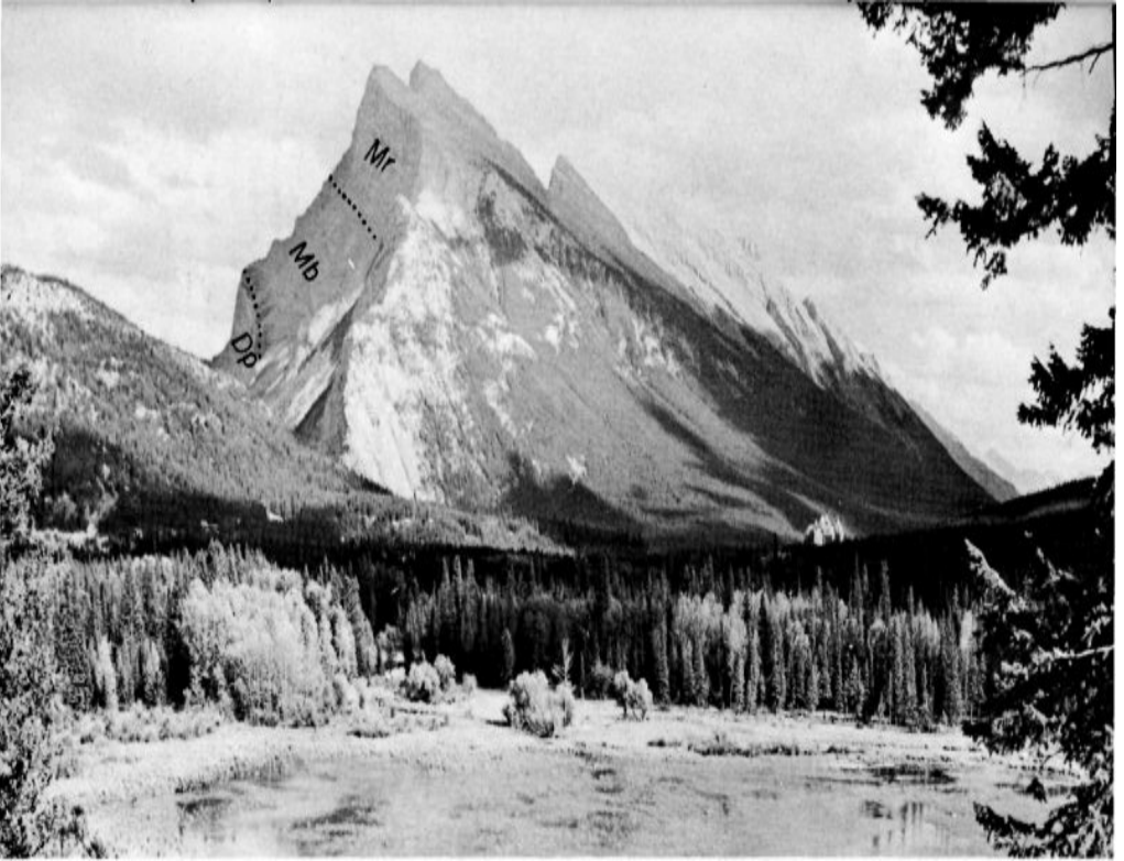
Figure 8. Mount Rundle, Banff. The layers of the Mississippian Rundle formation dip westward into the Spray River valley. The peak is Rundle limestone, the same rock formation from which Turner Valley oil and gas field, southwest of Calgary, has produced for many years. Mr—Rundle limestone; Mb—Banff shales; Dp—Devonian Palliser limestone cliffs.
