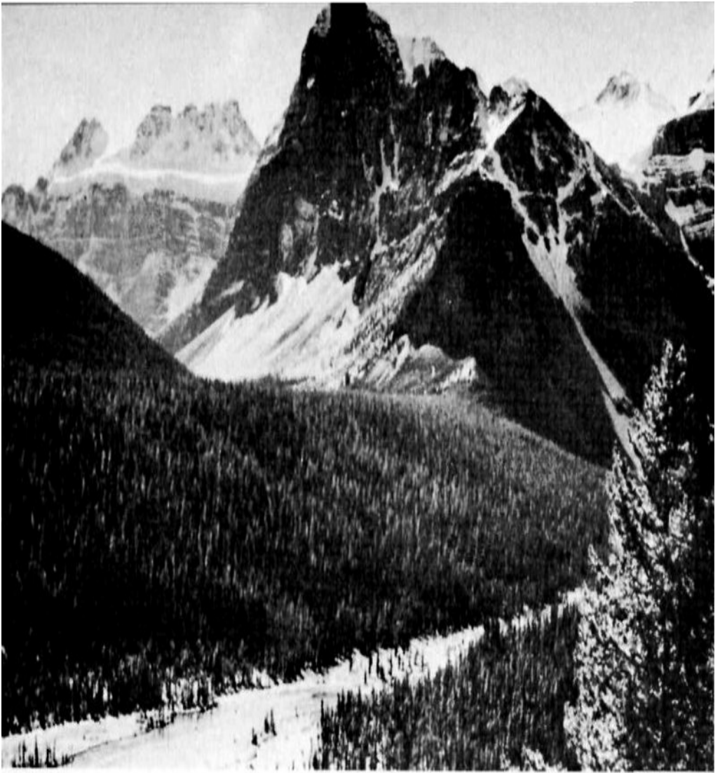
Figure 17. Mountains along the Continental Divide from the road to Moraine Lake. The terrace on which the road is built is the same as that on the opposite side of the valley. It is the remnant of an earlier glacial valley into which the stream has cut its present course, leaving the tributaries in hanging valleys.
