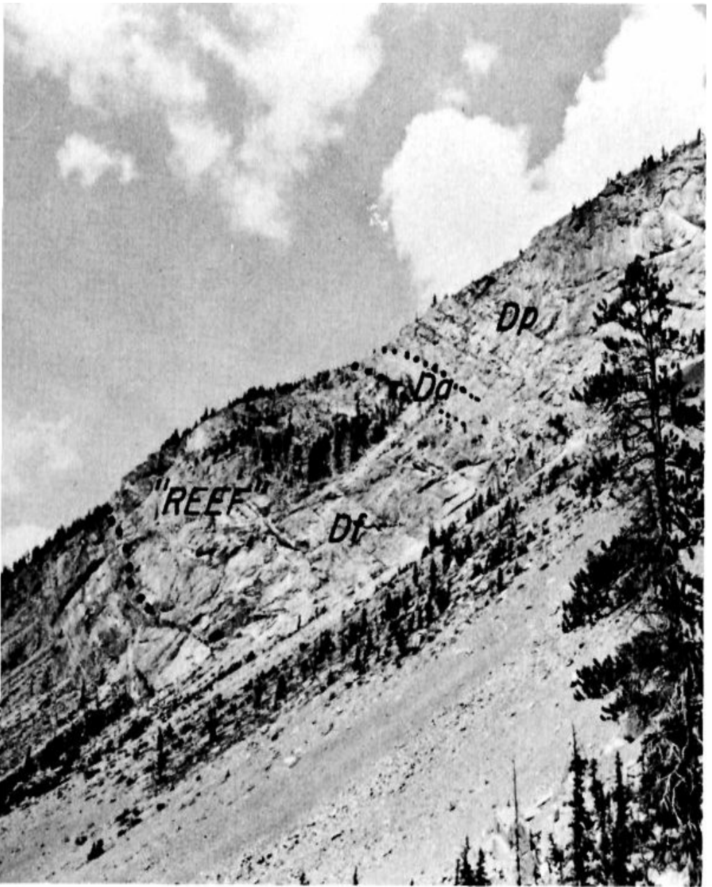
Figure 7. A massive Devonian white dolomite reef in the 'big hill', Sunwapta Pass, Banff-Jasper highway. This is the same type of structure as that from which oil is produced at Leduc, Redwater, Golden Spike and other fields in Alberta. Dp—Palliser limestone; Da—Alexo; Df—Fairholme.
