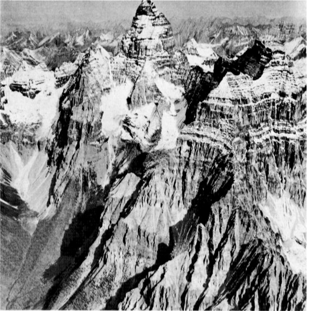
Figure 20. Mount Assiniboine. This peak, like the famous Matterhorn, was formed by cirques cutting into the mountain from all sides.
