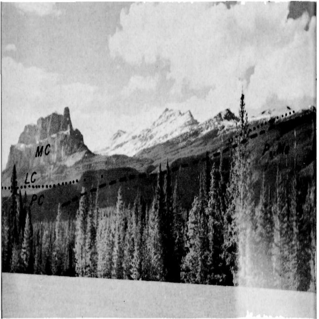
Figure 9. Mount Eisenhower as it appears today. Above the Castle Mountain thrust are Precambrian (PC) and Cambrian (LC and MC) rocks that have ridden up over late Palaeozoic (P) and Mesozoic (Me) rocks.
