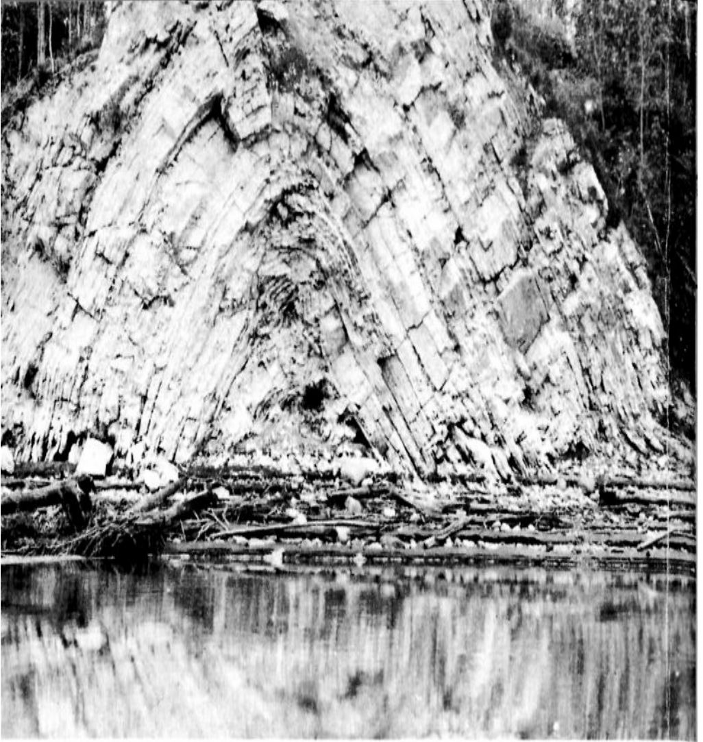
Figure 11. Rock arch or anticline.
