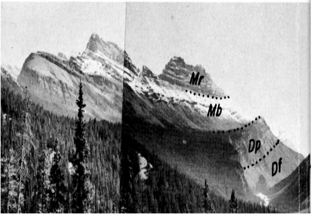
Figure 12. Cirrus Mountain, Banff-Jasper highway, as seen from near Sunwapta Pass. The rock layers bow down gently under the peak in the form of a syncline. Mr—Mississippian Rundle limestone; Mb—Banff shale; Dp—Devonian Palliser limestone; Df—Devonian Alexo and Fairholme.
