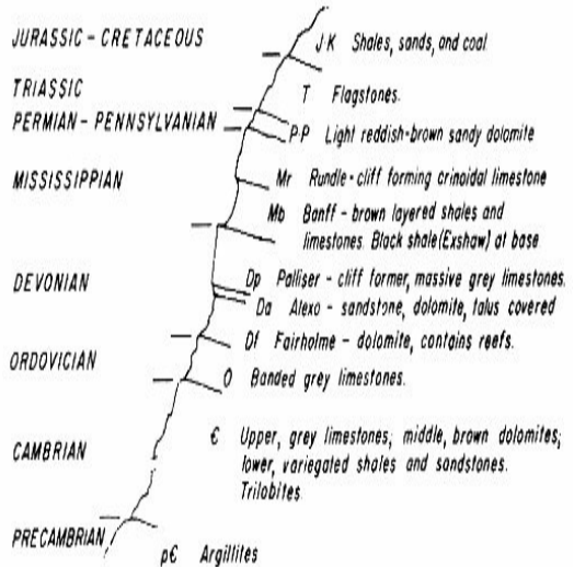
Figure 27. Diagrammatic section across the mountains from the Continental Divide at the headwaters of west flowing Simpson River and the east entrance to Banff National Park. Mount Rundle, as seen from the Hoodoos Viewpoint illustrates the alternating limestone cliffs and layered shale sequence typical of the Front Ranges of the Rocky Mountains east of Mount Eisenhower.
