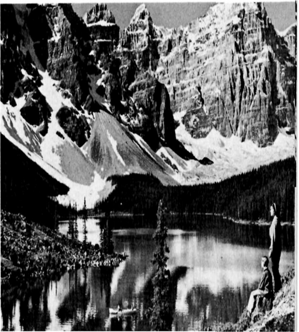
Figure 30. Moraine Lake in the Valley of the Ten Peaks near Lake Louise. The Peaks are cut in layered Lower Cambrian shales and quartzites. In the right background are recent glacial moraines left by glaciers that have retreated to the high peaks. Talus slopes fan outward and boulders of the rock slide dam the lake in the foreground.
