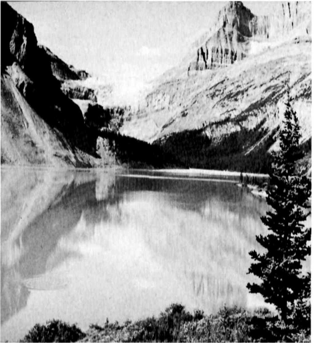
Figure 31. Bow Lake, with Bow Glacier in the distance, near the headwaters of Bow River. The mountains are made up of Lower Cambrian quartzites and shales overlain by Middle Cambrian limestones. Bow Glacier is a tongue of the Wapta ice-field, barely visible at the top of the glacier. Delta (right centre) is being built into Bow Lake by the stream of meltwater from the glacier as it carries glacial debris downwards.
