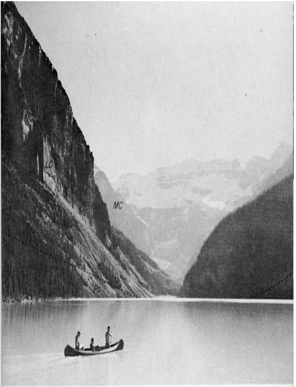
Figure 19. Lake Louise with Mount Victoria and Victoria Glacier in the distance. A cirque and moraines are visible below Victoria Glacier. Talus slopes (left centre) are composed of blocks of rock from the cliffs above. Pc—Precambrian; LC—Lower Cambrian; MC
