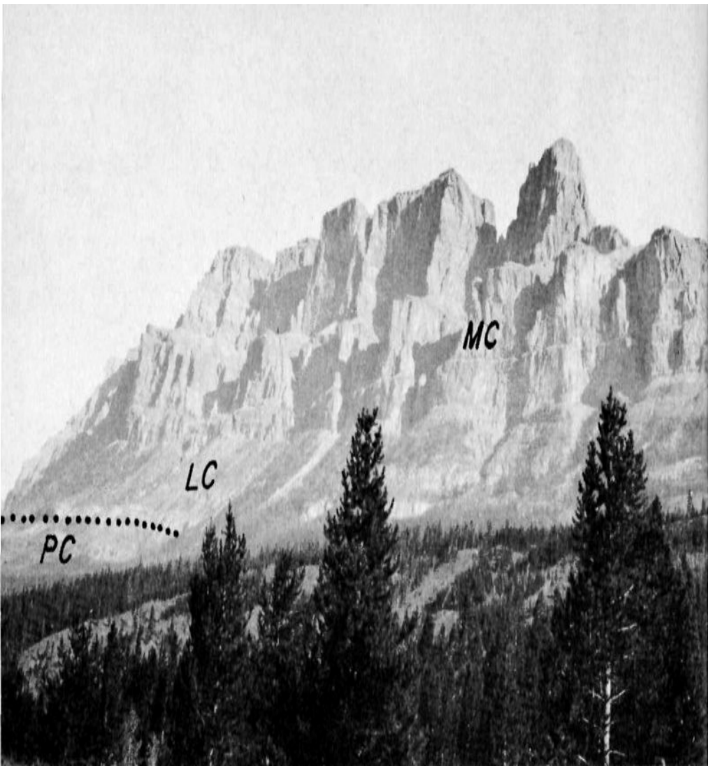
Figure 3. Mount Eisenhower from Vermilion Pass, Banff-Windermere highway. The vertical fractures that may be seen cutting the massive beds caused blocks of rock to fall away and left the sheer cliffs. The brown cliffs are Middle Cambrian limestone (MC), broken by the shales that carry fossil trilobites. LC—Lower Cambrian purple and green shales and pink quartzites; PC—Precambrian grey and purple shales.
