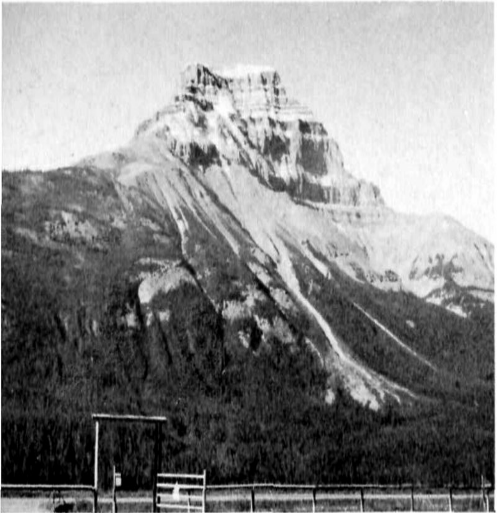
Figure 35. Mount Amery, one of the high peaks west of the Banff-Jasper highway. The peak is layered Upper Cambrian limestone resting on the Middle Cambrian of the great cliffs. The Lower Cambrian forms the rounded shoulders low on the mountain. Notice the glacier that caps the peak.
